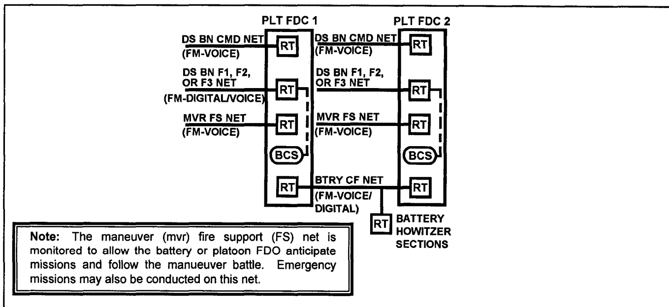
Figure 9-7. Battery radio nets
