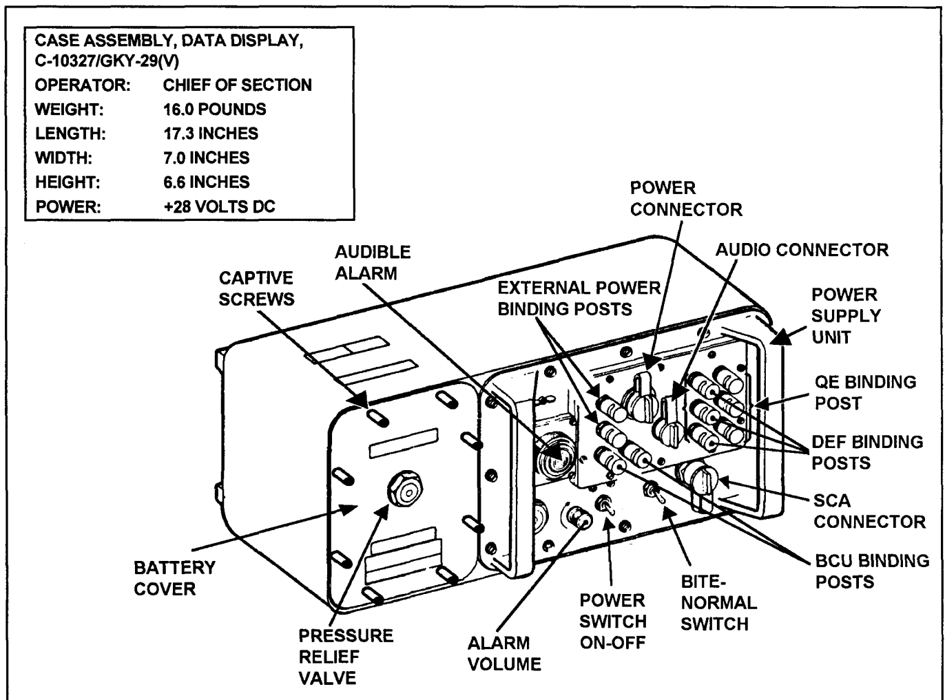
Figure L-3. Case assembly
